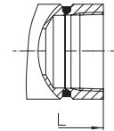
Fig. 600/601....2 with screwed sockets
