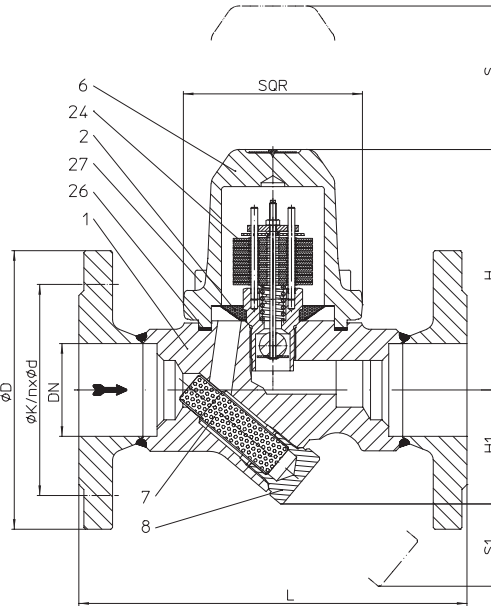
Fig. 601....1 with outside strainer (Y)
