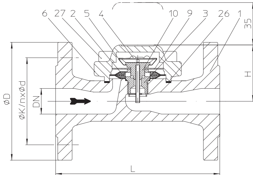
Fig. 616....1 with flanges
