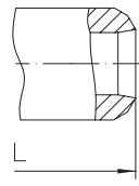
Fig. 610/612....4 with butt weld ends
