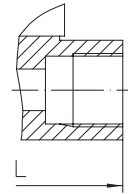
Fig. 610/612....2 with screwed sockets
