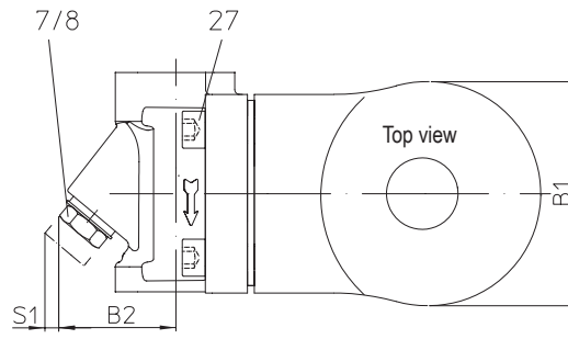
Fig. 634....2 (ANSI300) with screwed sockets - horizontal installation
