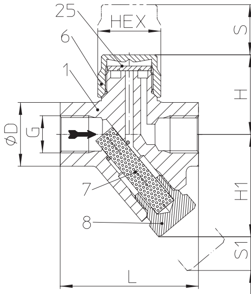
Fig. 641....1 with flanges
