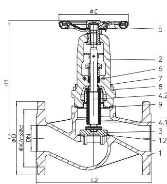
Fig. 141....153 1 1/2" - 6 one-piece stem
