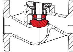
Regulating plug with soft seal Max. operating temperature 392°F / 200°C at PTFE + 25% carbon
