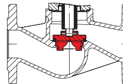
V-port regulating plug with soft seal Max. operating temperature 392°F / 200°C at PTFE + 25% carbon
