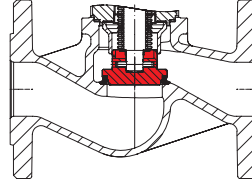
Plug with soft seal Max. operating temperature 392°F / 200°C at PTFE + 25% carbon
