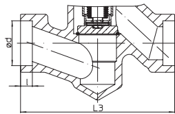
Fig. 149....111....3 / ....112.... with socket weld ends
