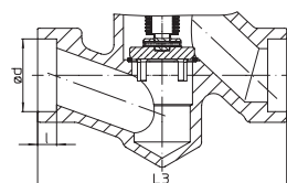
Fig. 149....153....3 / ....154....3 with socket weld ends
