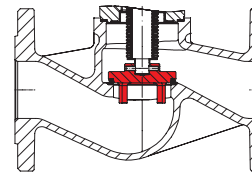
V-port plug with soft seal Max. operating temperature 392°F / 200°C at PTFE + 25% carbon
