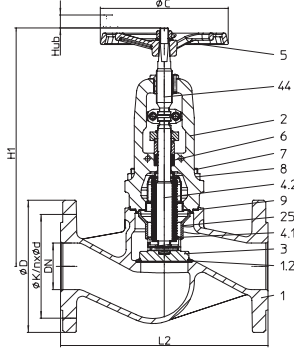
Fig. 141....112 1 1/2" - 6 two-piece stem
