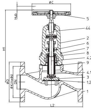
Fig. 141....154 1 1/2" - 6 two-piece stem
