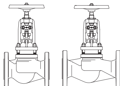
Fig. 141 One-piece stem
