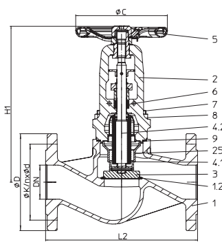
Fig. 141....111 1 1/2" - 6" one-piece stem
