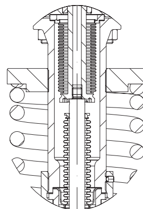
Bellows seal NPS 1"
