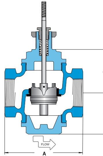
Stem In-to-Open (normally closed)
